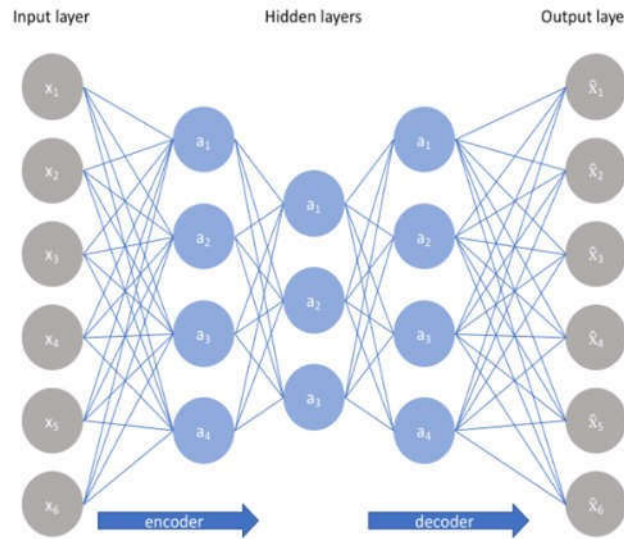
Figure 4. Autoencoder Model
